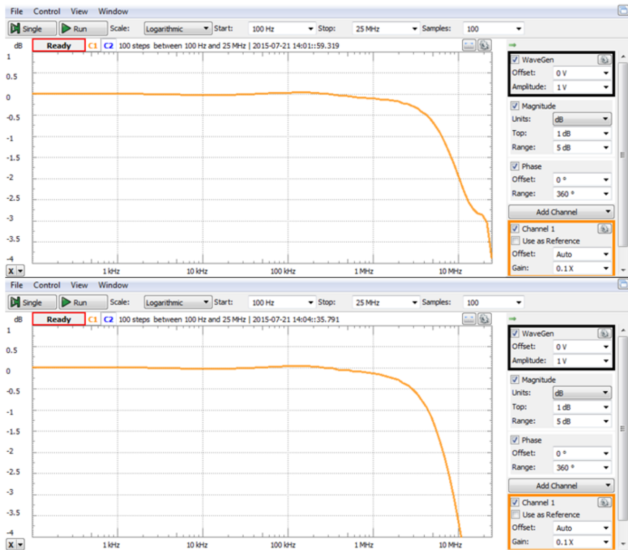
Figure 21. AWG spectral characteristics. With Analog Discovery BNC Adapter and BNC cable from AWG to Scope (up). With the wire kit (down).
