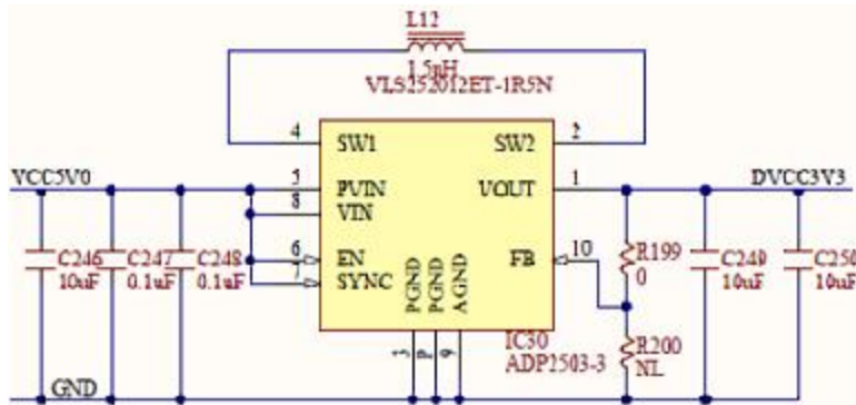
Figure 32. 3.3V internal digital supply.
