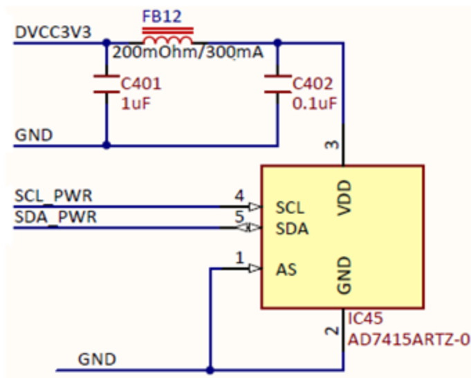
Figure 34. Temperature measurement.
