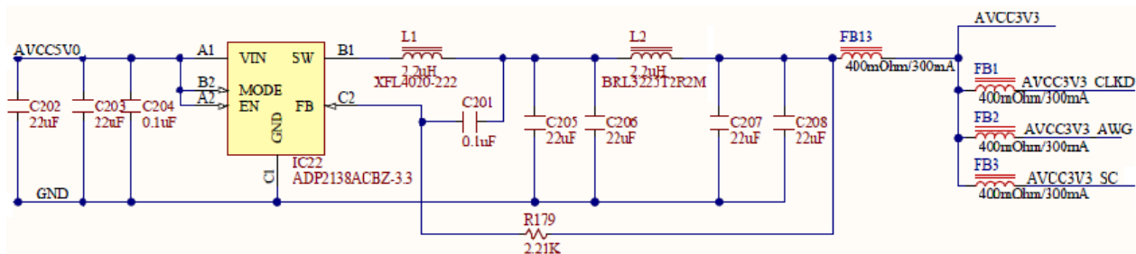
Figure 27. 3.3V internal analog power supply.
