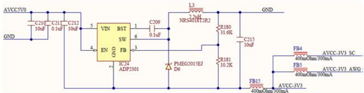
Figure 29. -3.3V internal analog power supply.
