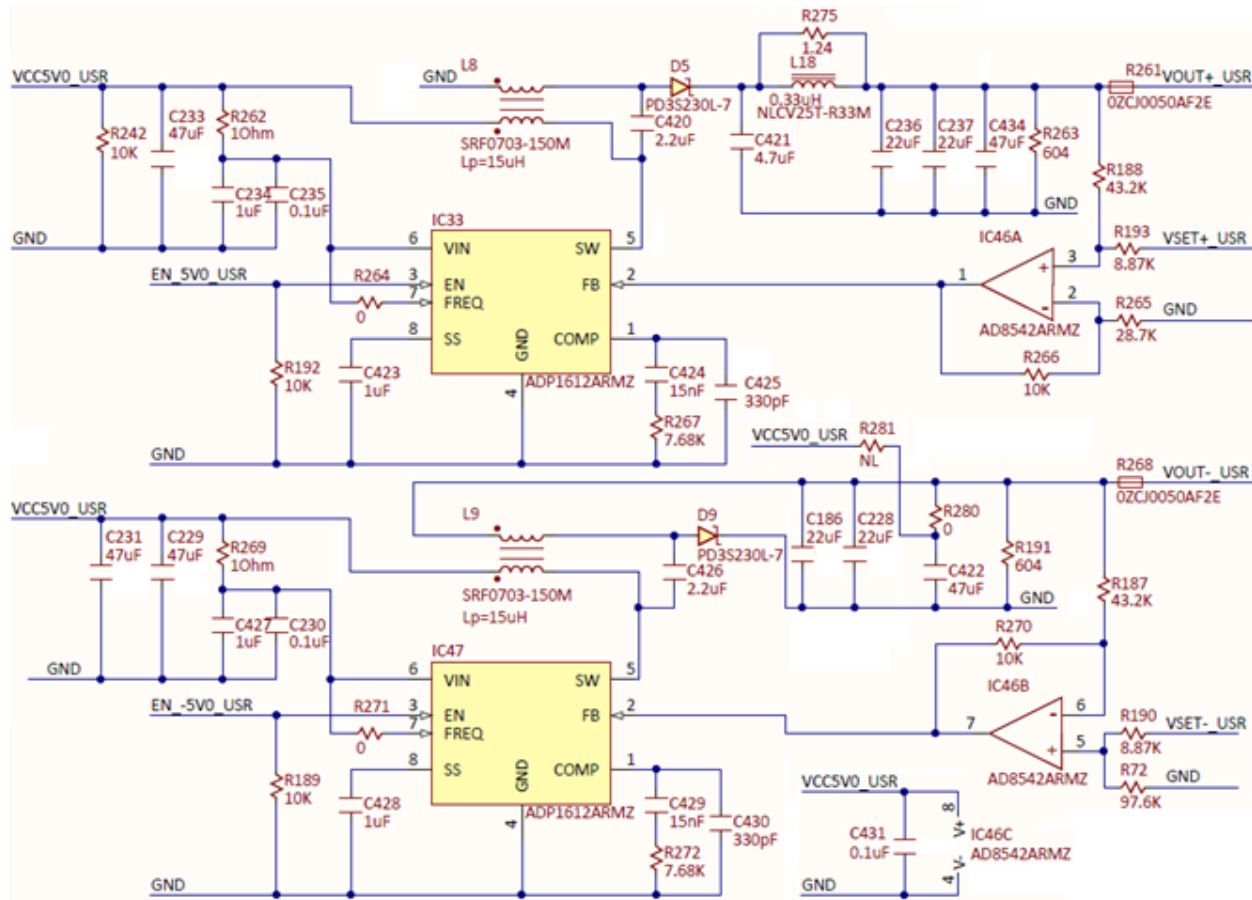
Figure 26. User power supplies.
