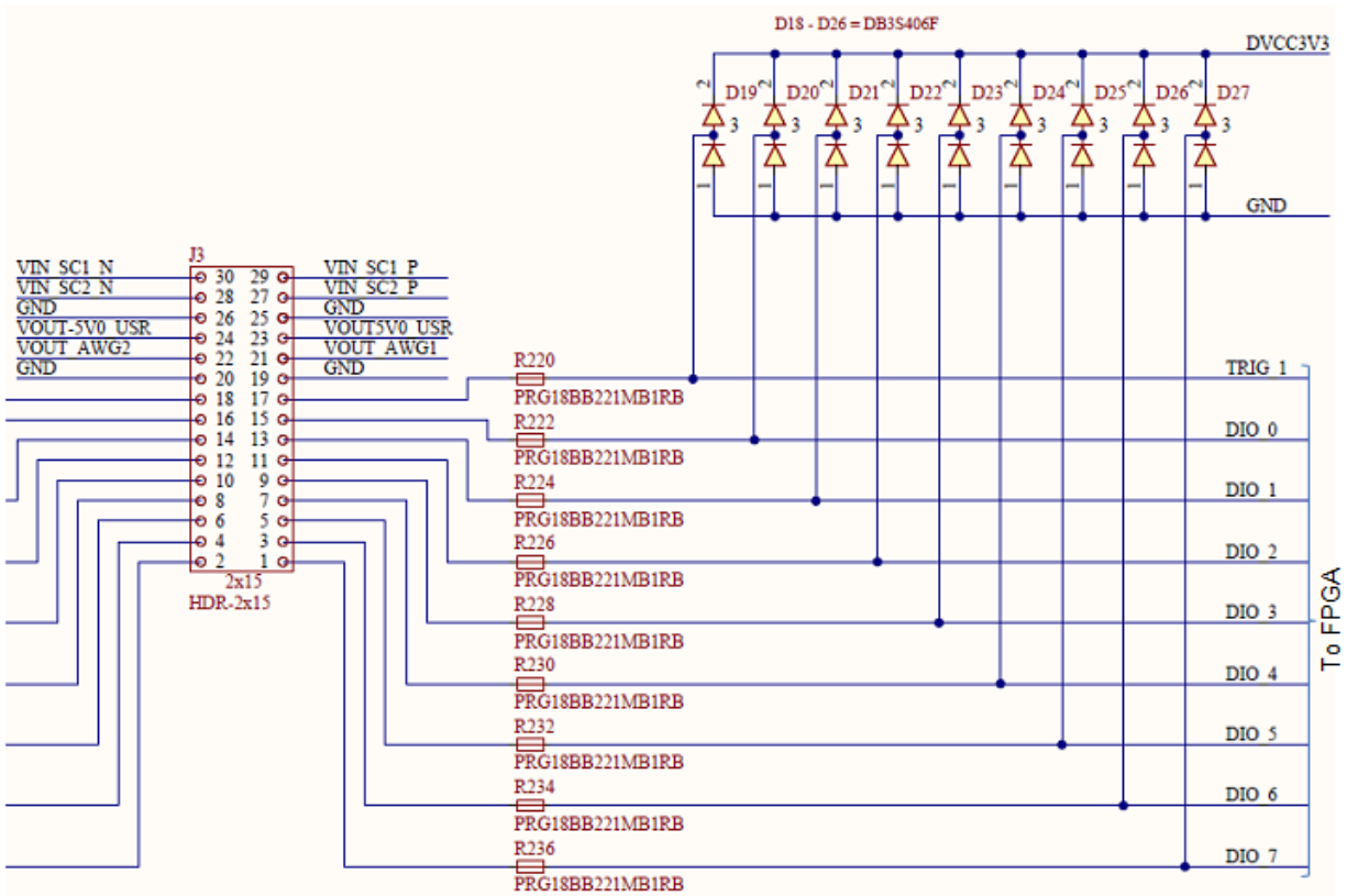
Figure 22. Digital I/O.
