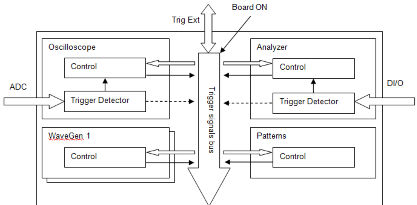
Figure 35. FPGA configuration trigger block diagram.
