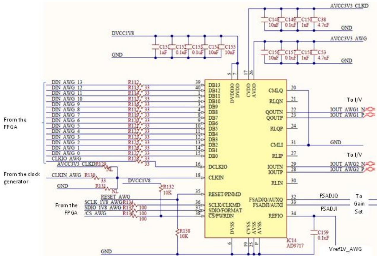
Figure 15. DAC
