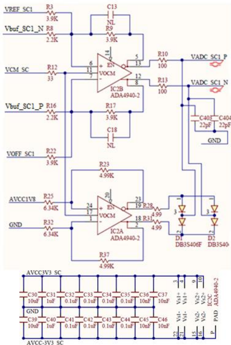
Figure 6. Scope driver.
