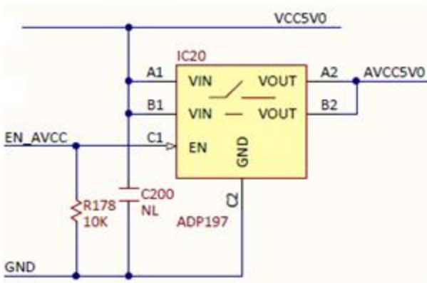
Figure 24. Analog Supplies control.
