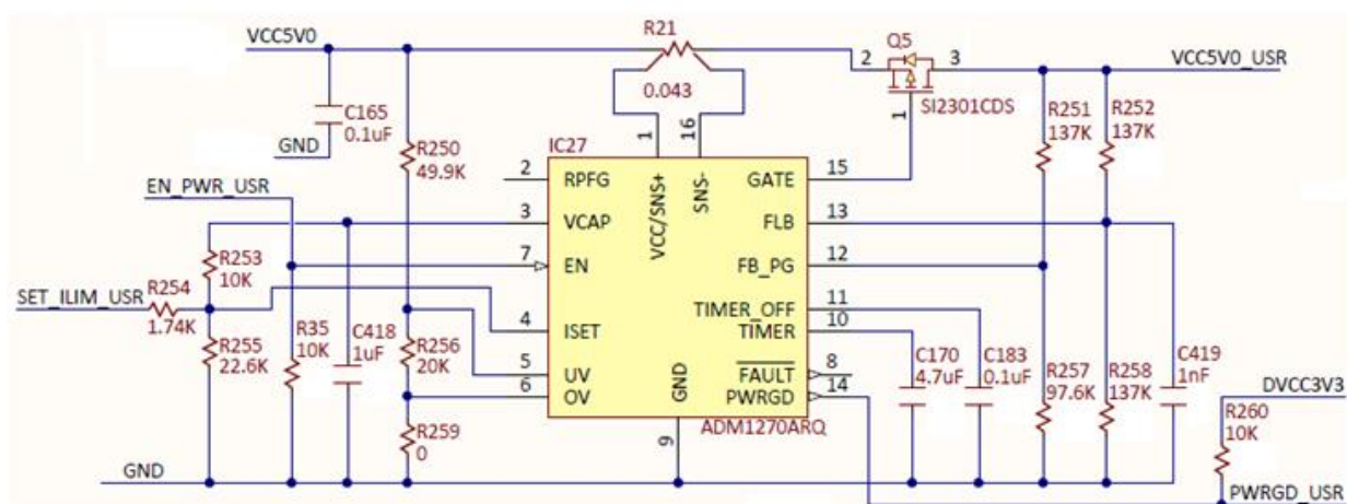
Figure 25. User supplies control.
