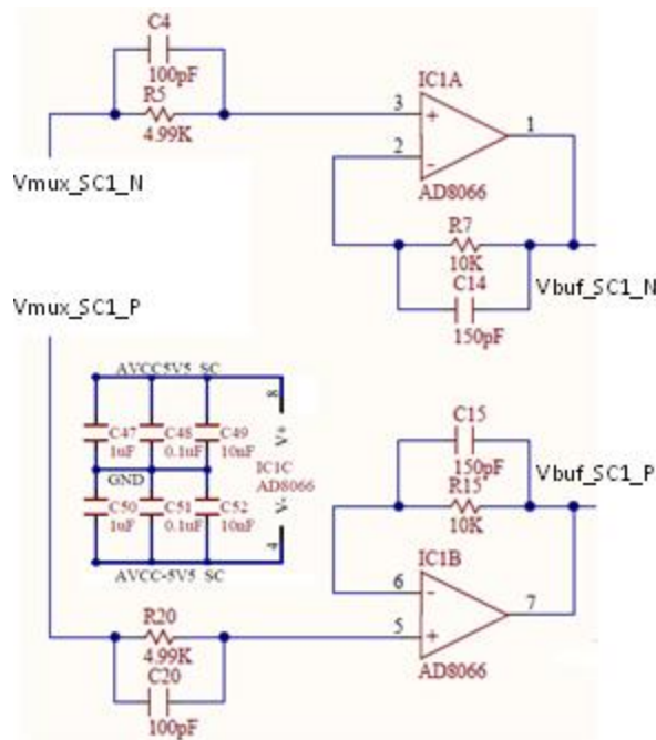
Figure 4. Scope buffer.
