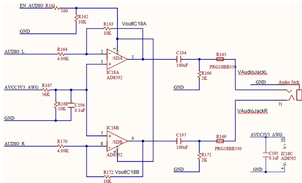
Figure 20. Audio.
