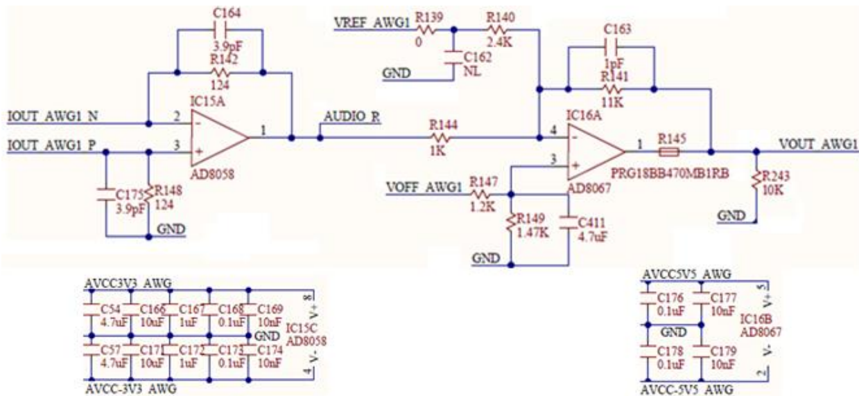
Figure 19. AWG I/V and out.
