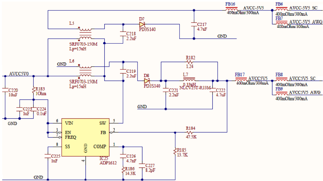
Figure 30. ±5.5V internal analog supplies.
