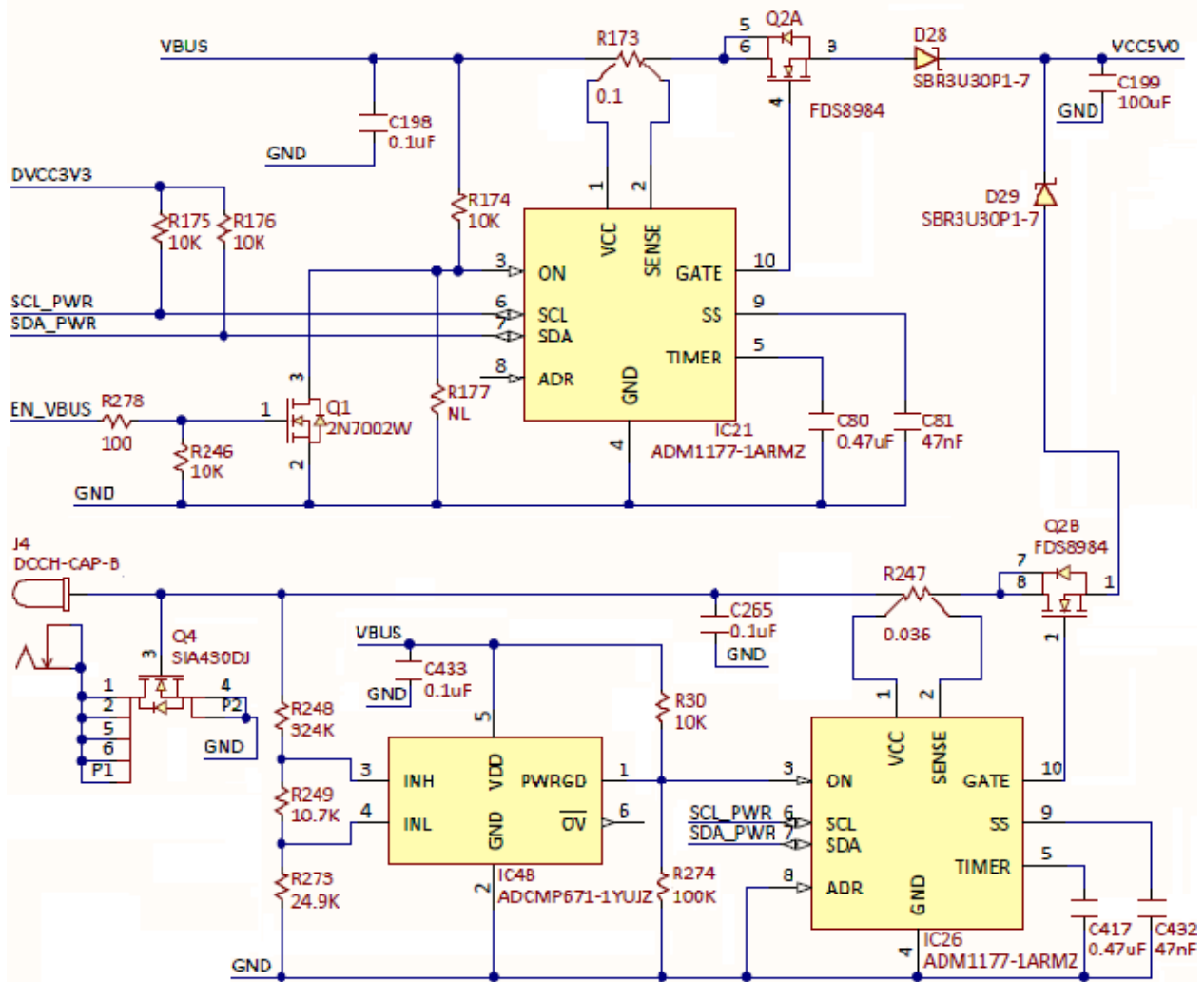
Figure 23. USB power control.
